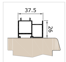
Adapterschiene ADS26Z
