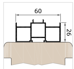
Adapterschiene ADS26ZK
